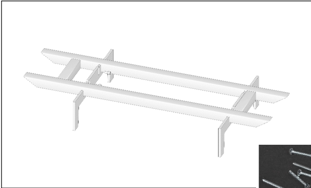
Montage FüÙe am Gestell Assembly of legs to the frame
